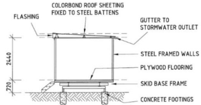
TYPICAL CROSS SECTION 1:100
